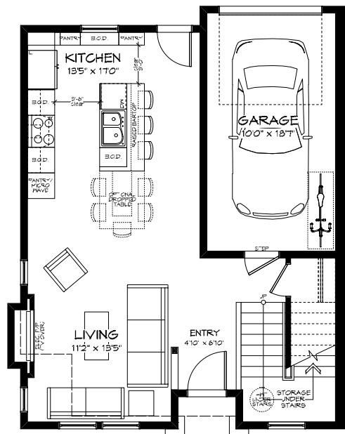
○ Typical Main Floor Plan (Units 1-5) 0 5 10 FT
